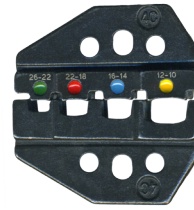
T-DIE-4C Insulated Terminals - Double Crimp
